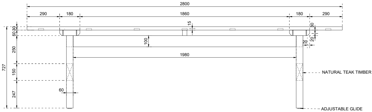
FRONT VIEW
